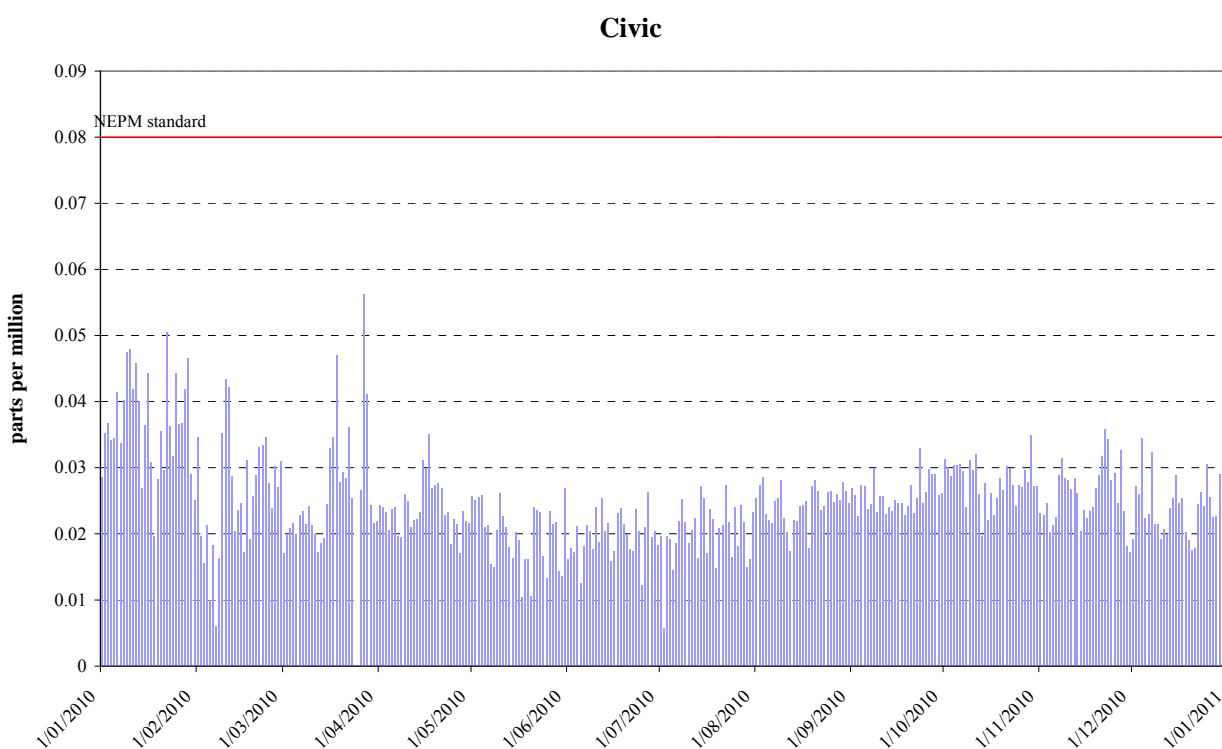
Figure 8: Daily max for 4 hours O 3 - Civic
