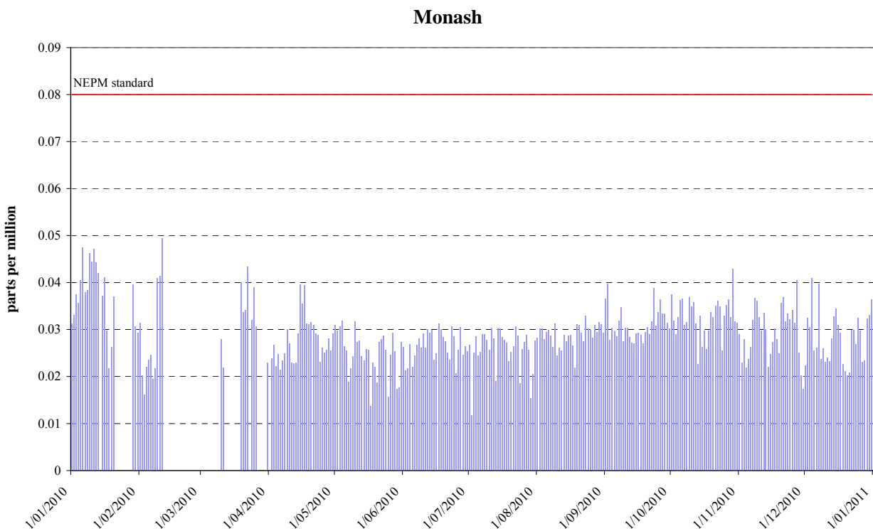
Figure 7: Daily max for 4 hours O 3 - Monash
