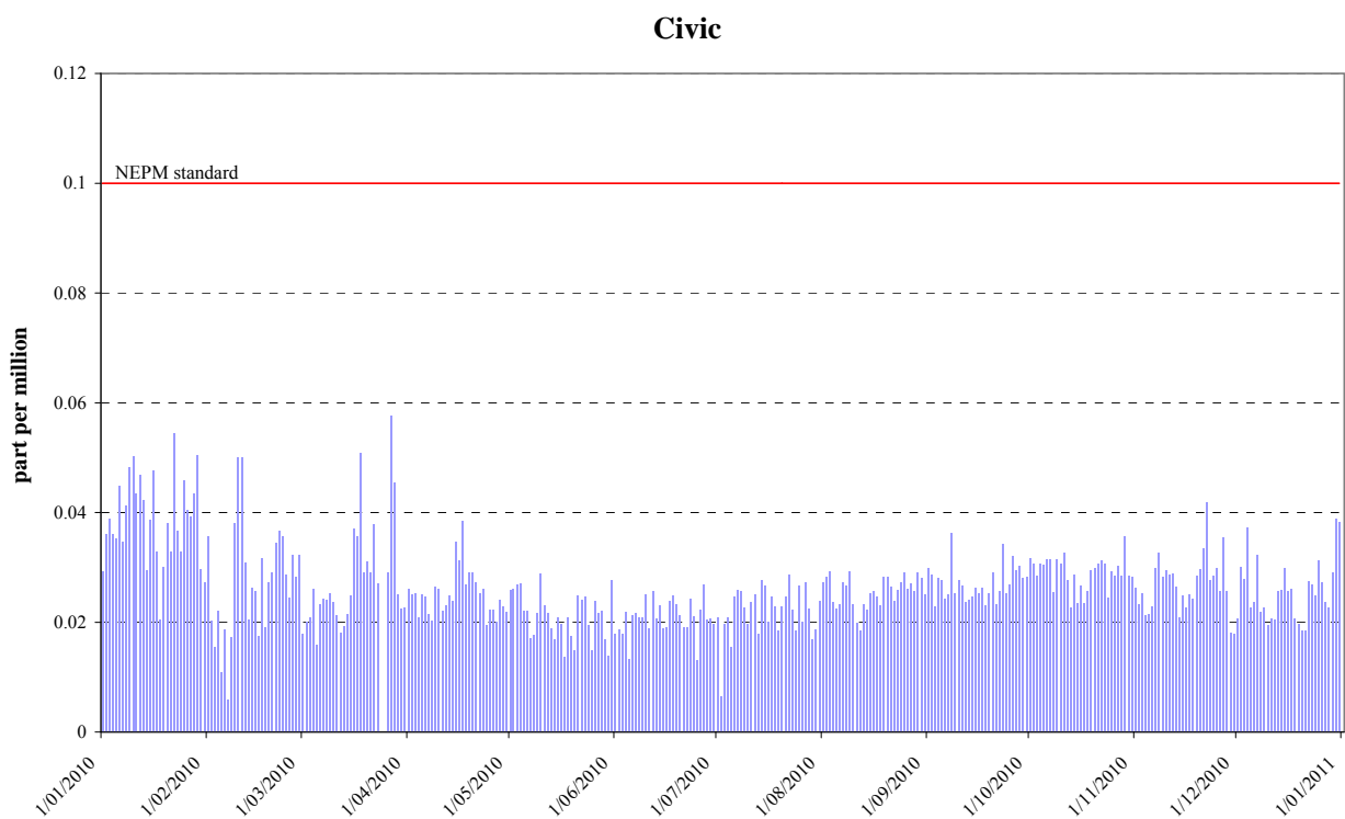
Figure 6: Daily max for 1 hour O 3 – Civic
