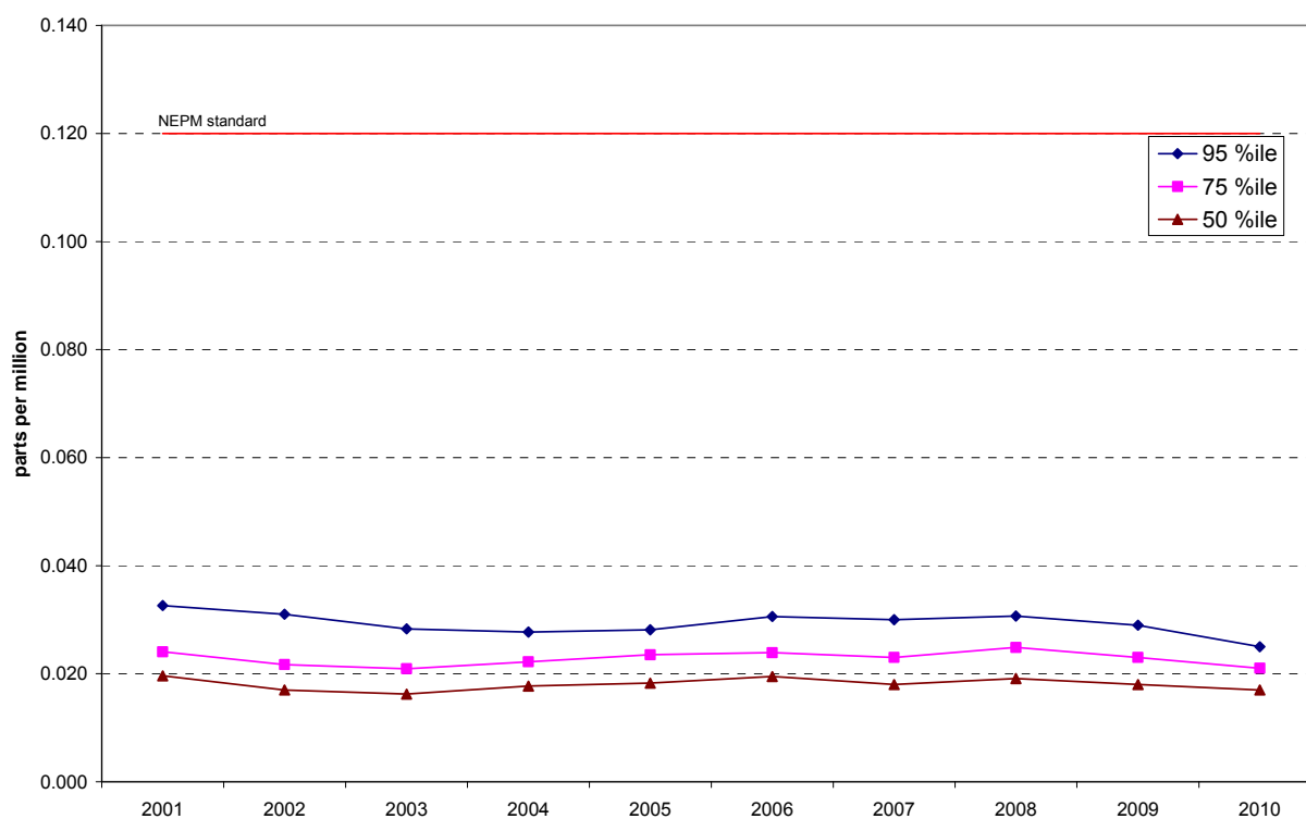
Figure 14: Statistical summary for daily maximum 1-hour NO 2 Monash 2001 – 2010
